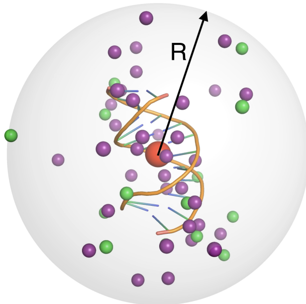
Figure 4.1.: Example of the restraining sphere used to set the simulation volume and ion concentration in ISEXI (gbion) model. Purple and green spheres are \text{Na}^+ , and \text{Cl}^- ions, respectively. The grey sphere of radius R with its center near the center of mass of the DNA fragment illustrates the simulation volume. The red sphere denotes the center of the restraining sphere.
